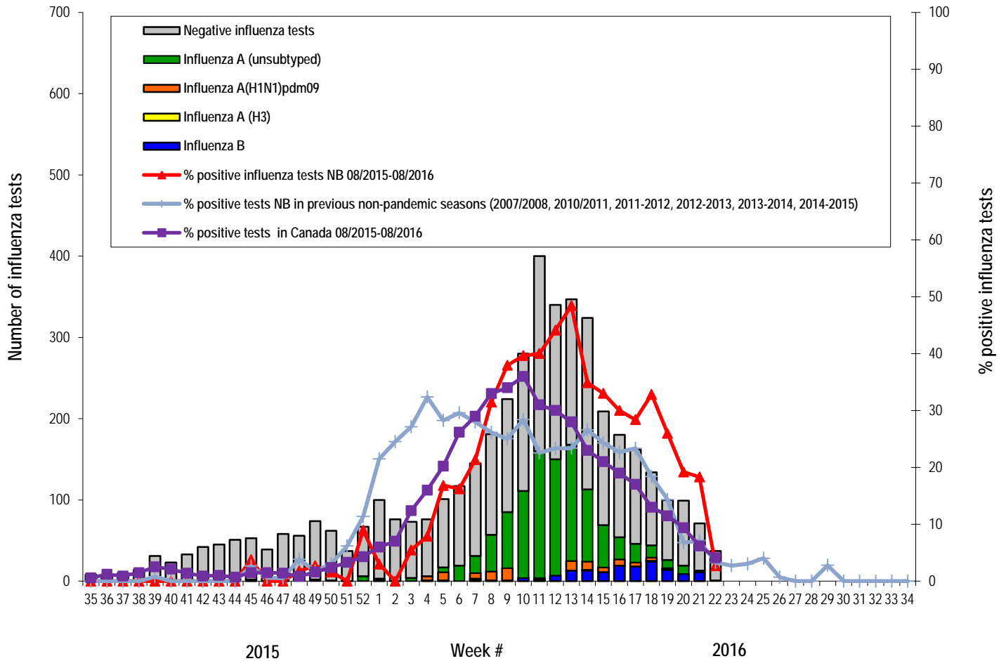
Graph 1: Number and percent of positive influenza specimens in New Brunswick by week, up to June 4 2016 (data source: G. Dumont Lab results)
