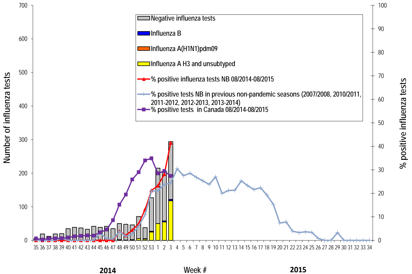
Graph 1: Number and percent of positive influenza specimens in New Brunswick by week, up to January 24 2015 (data source: G. Dumont Lab results)
