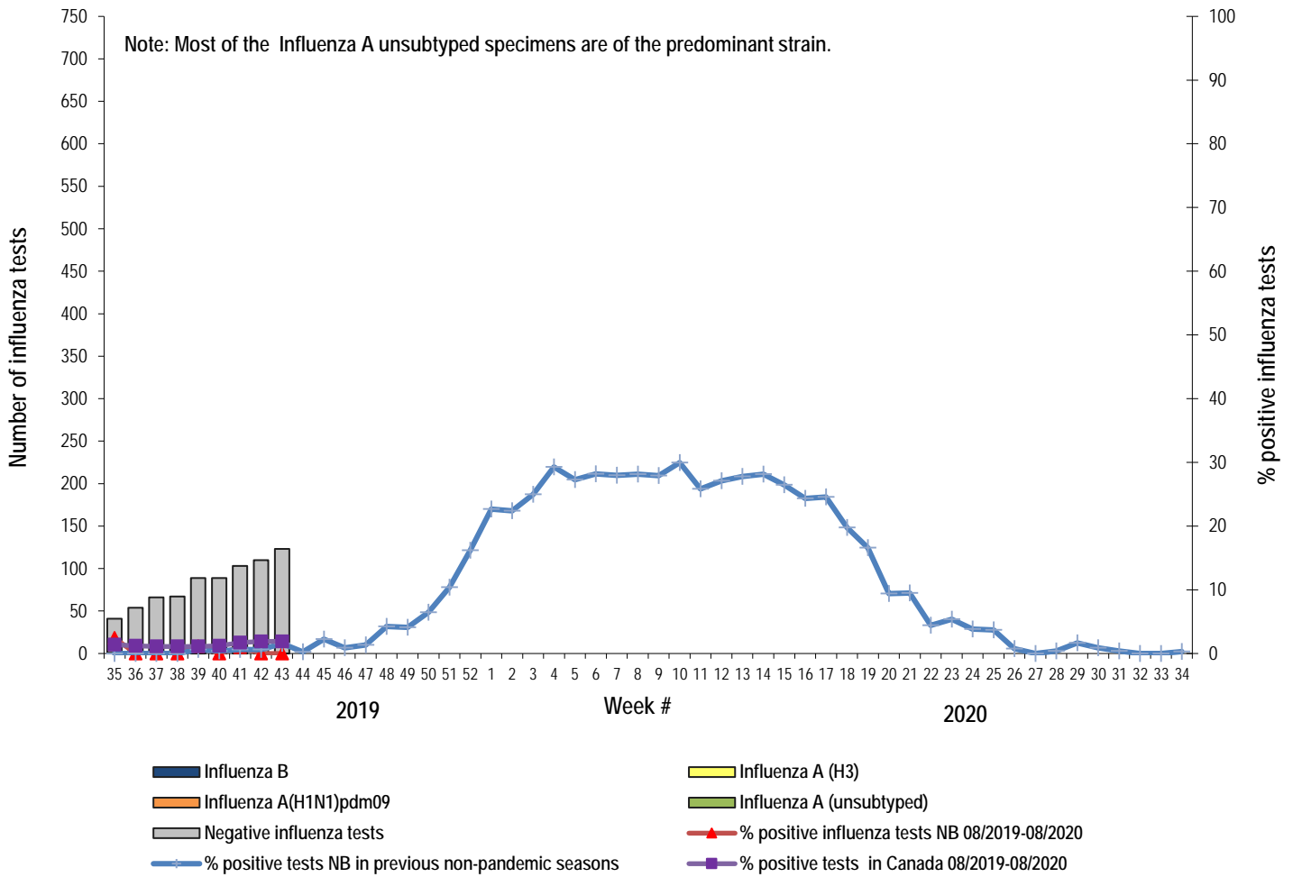
Graph 1: Number and percent of positive influenza specimens 2 in New Brunswick by week, up to October 26, 2019 (data source: G. Dumont Lab results)
